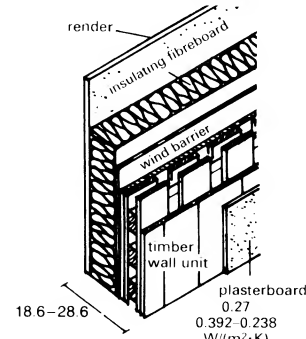
⑭ Timber unit wall (Lignotrend) 0.27 0.392-0.238 W/(m 2 ·K)
